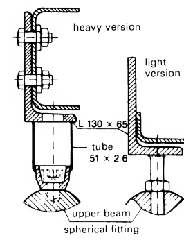
⑧ Purlin fixings
